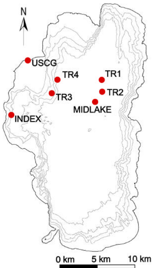
Figure 11.4.5.1-1. Bathymetric map of Lake Tahoe with a contour interval of 100 m. The 4 NASA rafts are labelled TR1, TR2, TR3 and TR4. Also shown is the US Coast Guard station (USCG), Midlake and Index stations. A variety of atmospheric measurements are made at the USCG and a variety of water properties are measured at the Midlake and Index stations.
