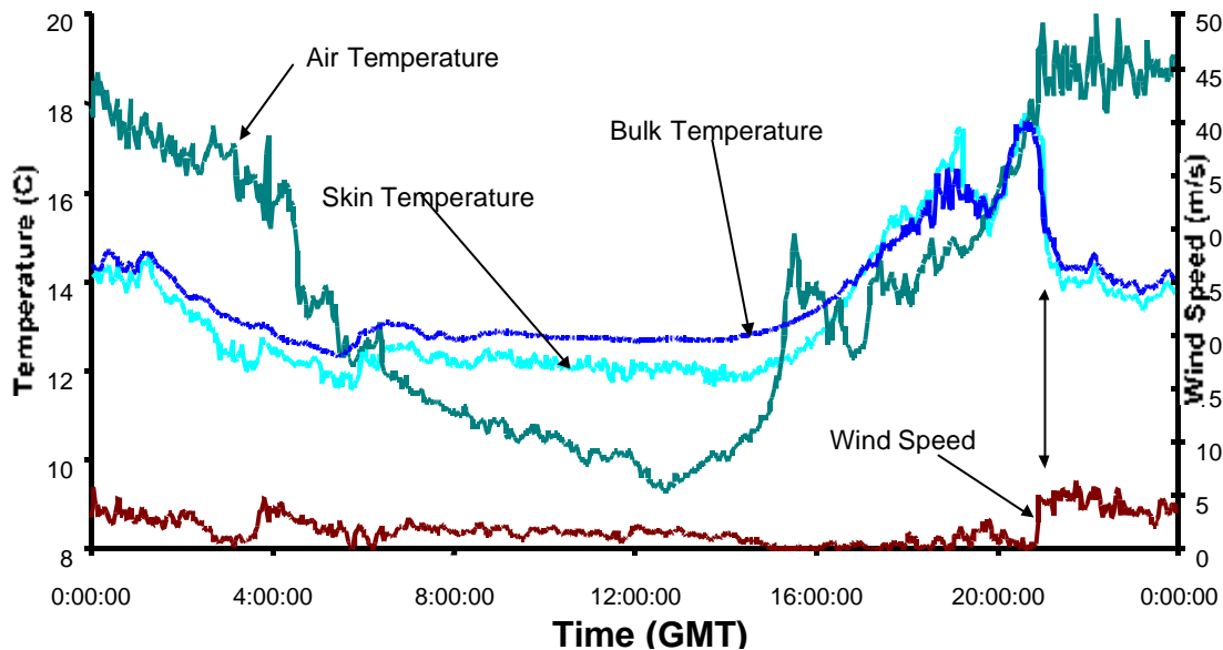
Figure 11.4.5.1-4. Variations in the bulk-, skin-, air-temperatures and wind speed on June 7, 2001 at L. Tahoe.
