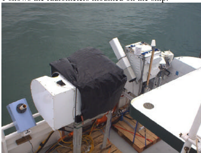
Figure 9.3.2.2-1 View from above of the radiometers mounted on the R/V Walton-Smith. From fore to aft, they are the SISTeR, ISAR (hidden), CIRMS, M-AERI and DAR011
