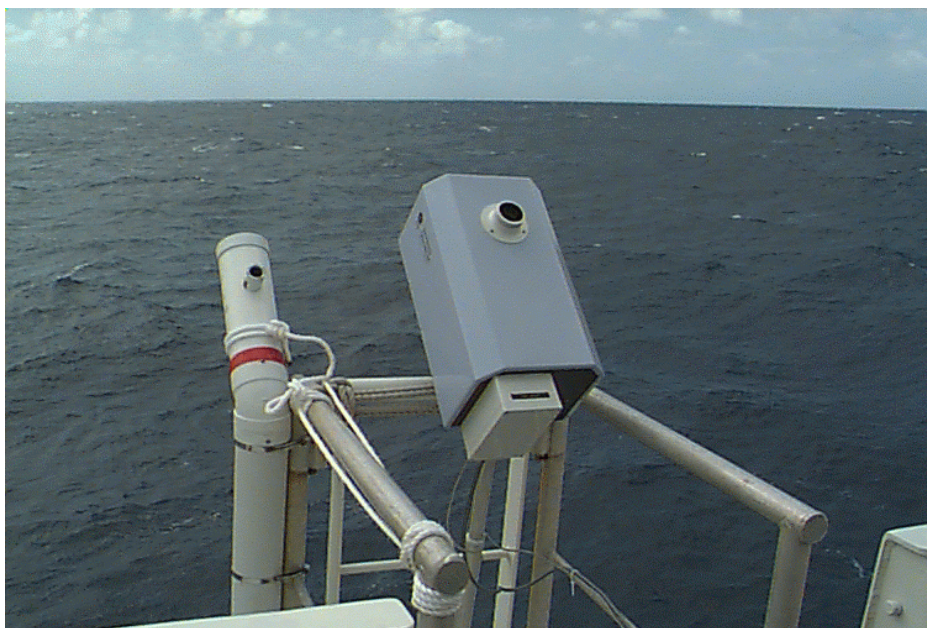
Figure 9.3.3.1-1: The DAR011 radiometer, mounted on the RV Franklin, used for validation activities based in Hobart. (Photograph from CSIRO)
