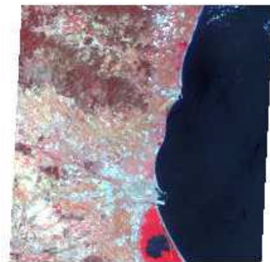
Figure 11.4.4.2-1 ASTER image of the Valencia study area (30 th June 2000)
