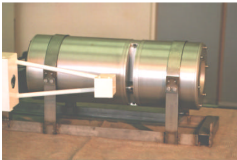
Figure 9.2.1.1-1 The Infrared Autonomous SST Radiometer (ISAR) shown together with the optical rain gauge in place. The rain gauge is used to control the opening/closing of a shutter system that seals the instrument from rain and sea spray during bad weather. The shutter is open in this picture revealing the small viewing aperture and scan drum assembly.
