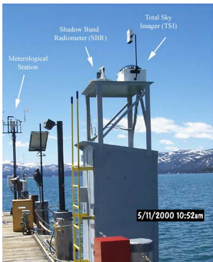
Figure 11.4.5.1-3. Yankee Total Sky Imager (TSI) and Yankee Multi Filter Rotating Shadowband Radiometer (MFRSR) located above the gauging station on the US Coast Guard Pier. A full meteorological station is also located on the pier and maintained by UCD.
